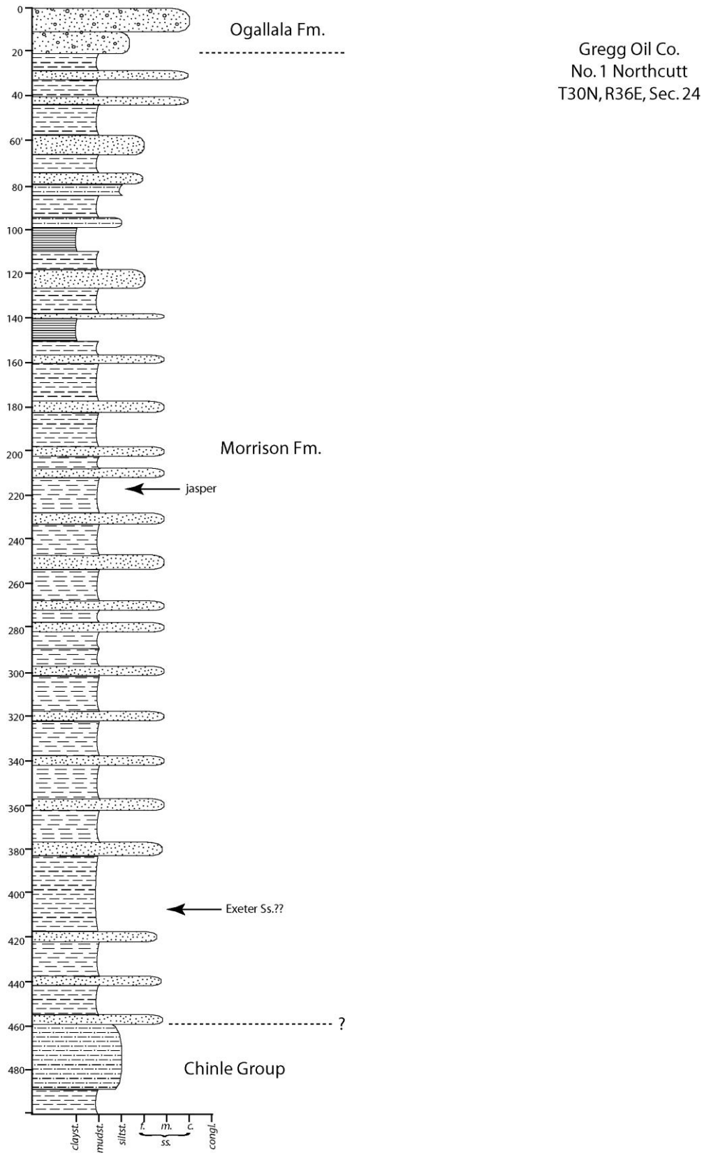
Figure 6. Gregg Oil Co. No. 1 Northcutt interpreted stratigraphic column.
